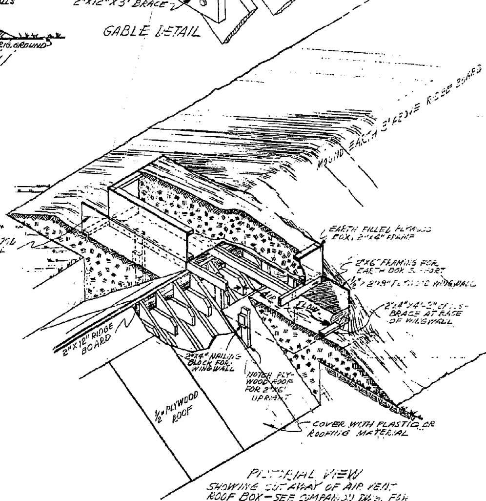
0.2. A-Frame Expedient Shelter, Alternate Air Vent Design.
